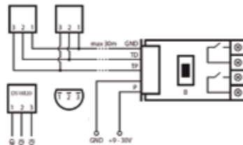
Connection to DS18B20 temperature sensors
