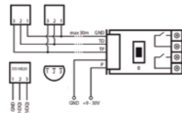
Connection to DS18B20 temperature sensors
